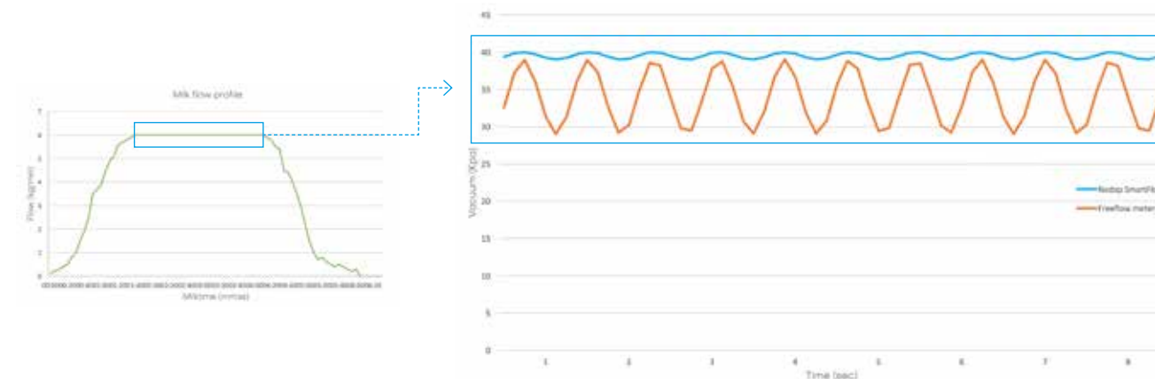
Vacuum fluctuations at flowrate 6 kg/min of the Nedap SmartFlow compared to a conventional freeflow milk meter. ▲
