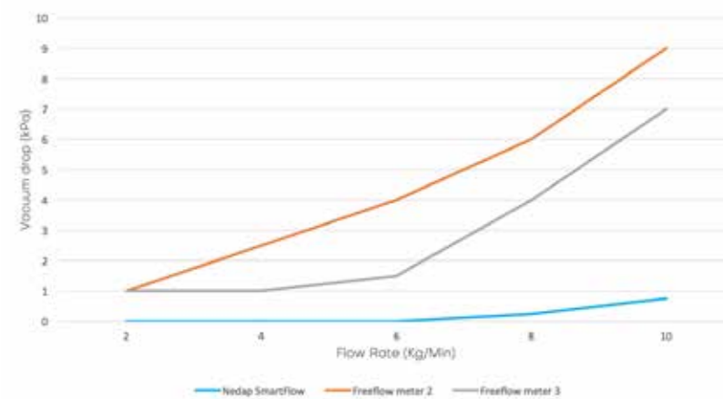
Vacuum drop in relation to flow rate of the Nedap SmartFlow compared to two conventional freeflow milk meters. ▲
